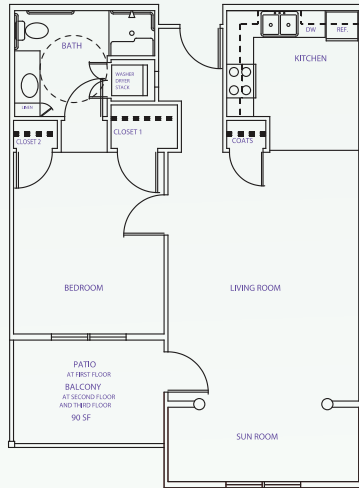
804 SQUARE FEET PLUS BALCONY = 90 SF One Bedroom Apartment HANDICAPPED ACCESSIBLE
