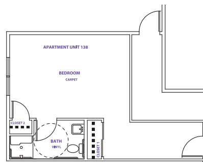
401 SQUARE FEET One Bedroom Apartment HANDICAPPED ACCESSIBLE
