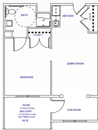
575 SQUARE FEET PLUS BALCONY = 90 SF One Bedroom Apartment HANDICAPPED ACCESSIBLE
